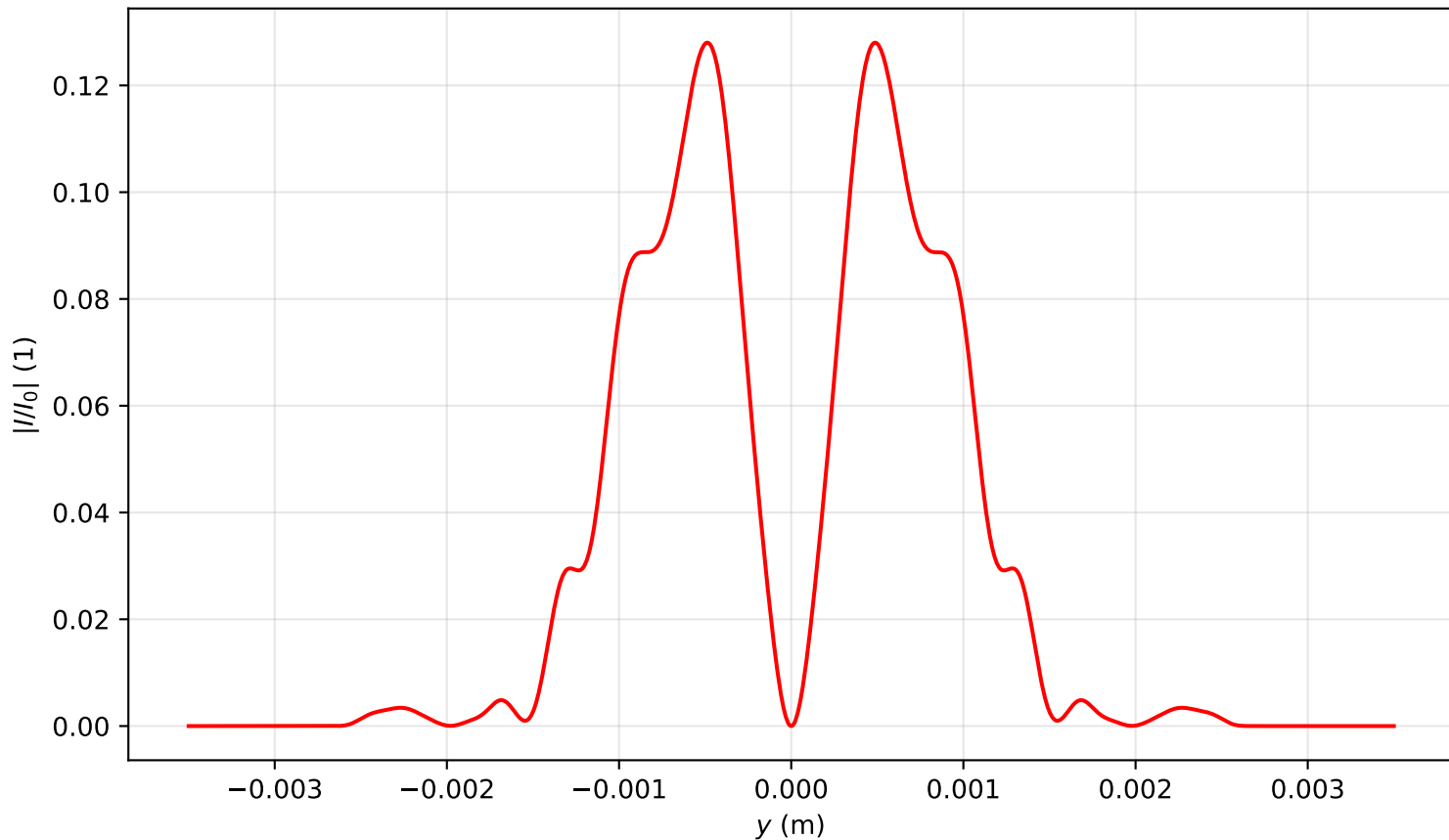
Intensity profile I(x=0, y, z=2.946)/I_0 , \text{Pin}=7.0\text{Pcr} , artificial time
